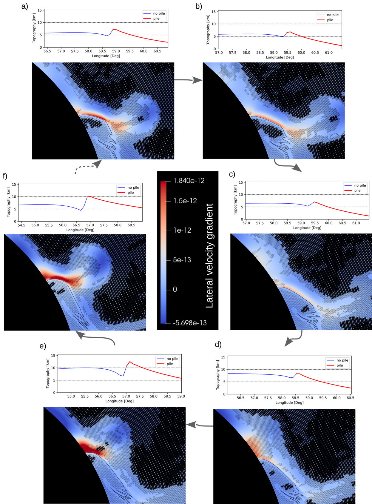
Fig. 5. CMB topography and lateral velocity gradients of v_\psi during a cycle of plume initiation and growth. A plume being pushed towards the pile interior increases the local pile edge thickness, while pulling the pile margin along the TBL in the flow direction, thereby reducing the lateral velocity gradient and the topographic depression (panels (a)-(c)). As soon as the upward plume pull decreases and no longer supports the thickened pile, the pile edge starts to collapse and spread along the CMB in a direction opposite to the TBL flow (panels (c) to (e)). This increases compression in the TBL wedge significantly, which amplifies CMB topography. It also thickens the lower thermal boundary layer, triggering a new plume (e). When the plume starts to rise, the lateral pile edge motion stops, the velocity gradients and CMB topography start to decrease (f), and the cycle starts anew.
