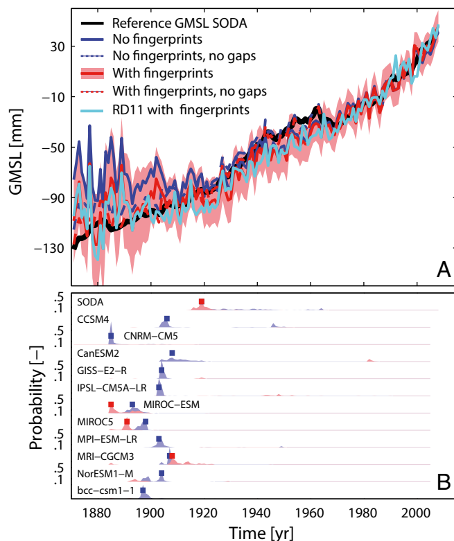
Fig. 2. Performance of the area-weighted average approach in ocean models. (A) Sensitivity of the area-weighted average technique in the SODA reanalysis (its reference GMSL is shown by the black line) to the four initial data sets: Gaps as in reality, no fingerprint corrections applied (dark blue); assuming a full record, no fingerprint corrections applied (dark blue dotted); gaps as in reality, fingerprint corrections applied (red, with shading noting its 1\sigma uncertainty); and assuming a full record, fingerprint corrections applied (red dotted) (see Fig. S3 for the respective curves from the 11 CMIP5-based synthetic sea level fields). The cyan curve represents a GMSL reconstruction with gaps as in reality and fingerprint corrections applied, but using the tide gauge subset from ref. 2. (B) Results of the Bayesian change point analysis (25) on the differences between each model specific reference GMSL and corresponding tide gauge reconstruction, without fingerprint corrections; red, with fingerprint correction) in each model. The change point analysis provides statistically the probability and timing of changes (shaded areas) in the relationship between the “true” model GMSL and its reconstruction. Tall, thin spikes suggest relative certainty in the timing of a change point, whereas wider spikes suggest more uncertainty in its timing. The red and blue squares mark the most probable timing from 500 iterations.
