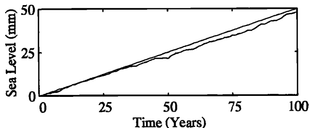
Figure 5. Cumulative sea level rise due to Antarctic ice mass changes for the loading model used to calculate displacements.
