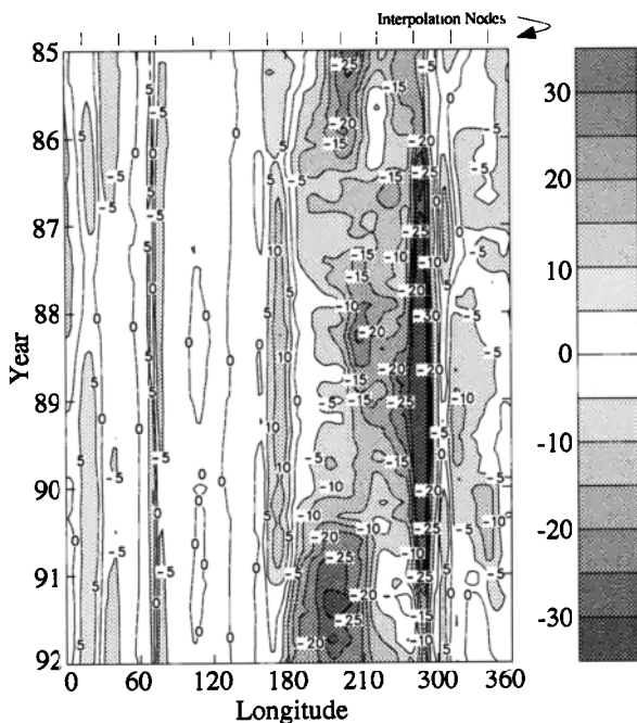
Figure 2. Time vs. longitude plot of meridional moisture transport across 70° S. Negative values indicate a southward directed moisture flux. Units are \text{kg m}^{-1} \text{s}^{-1} . The upper tick marks indicate interpolation nodes used to define the spatial variability of precipitation in the ice loading model (see text). Reproduced from Bromwich et al., 1995.
