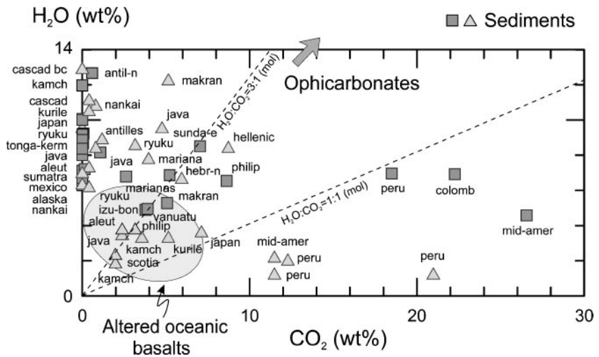
Figure 2 Estimates of the amount of \text{H}_2\text{O} in hydrates and \text{CO}_2 in carbonates in crustal columns being subducted. From Plank & Langmuir (1998) (squares) and Rea & Ruff (1996) (triangles). The shaded field represents altered MORB (Staudigel et al. 1996). Ophicarbonates after the data in Sciuto & Ottonello (1995) and Bonatti et al. (1974).
